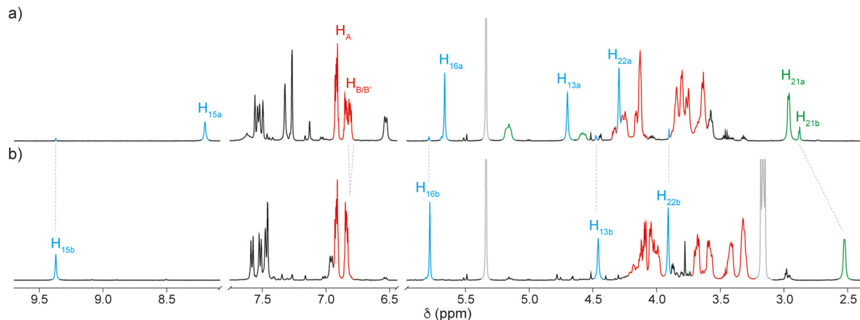
Fig. 2 Partial 1 H NMR spectra (500 MHz, CD 2 Cl 2 , 298 K) of a 95 : 5 mixture of rotaxane 1aH 2+ ·2PF 6 − and 1bH 2+ ·2PF 6 − (a) and the same sample after addition of 1 equivalent of tBu 4 NCl displaying mainly 1bH 2+ ·2Cl − (b). Signals are color-coded and numbered according to Scheme 1. The residual solvent and the tetrabutylammonium signals are color-coded in grey.
