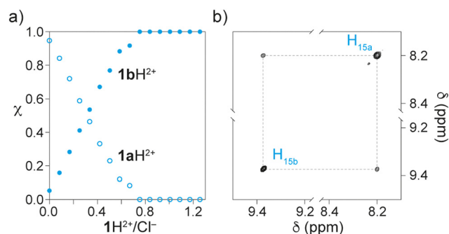
Fig. 3 (a) Titration of 1aH 2+ ·2PF 6 − with tBu 4 NCl. Molar fraction of 1aH 2+ (hollow circles) and 1bH 2+ (full circles). (b) Partial EXSY spectrum (500 MHz, CD 2 Cl 2 , 298 K, t_{\text{mix}} = 200 ms) showing the chemical exchange between the triazolium signals of 1aH 2+ (H 15a ) and 1bH 2+ (H 15b ).
