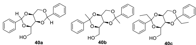
Fig. 26 Xylitol-based organogelators.
