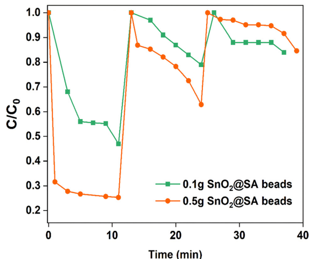
Fig. 12 Regenerative studies of 0.5 g and 0.1 g \text{SnO}_2\text{@SA} beads for 5 \mu\text{M} CR aqueous solution.
