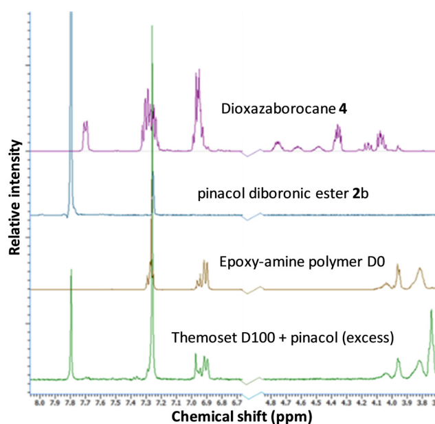
Fig. 8 ^1\text{H} -NMR spectra of epoxy-amine-dioxazaborocane D100 after chemical recycling via pinacol methodology (according to Fig. 7b).
