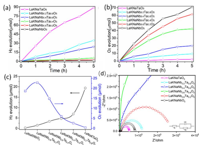
Fig. 7 Photocatalytic performance of LaKNbNb 1-x Ta x O 5 nitrated at 1123 K for 4 h ( x = 0, 0.2, 0.4, 0.6, 0.8, 1.0 ): (a) H 2 and (b) O 2 evolution as a function of time, (c) H 2 and O 2 evolution rates, and (d) EIS spectra recorded under visible light illumination. Reaction conditions for H 2 evolution: 150 mL of aqueous methanol (20 vol%), photocatalyst: 300 mg, co-catalyst: 0.5 wt% Rh, loading method: impregnation with H 2 reduction, light source: a 300 W xenon lamp ( \lambda \geq 420 nm), reaction cell: a top-irradiation cell with a Pyrex window. Reaction conditions for O 2 evolution: 150 mL of an aqueous 50 mM AgNO 3 solution containing 0.20 g of La 2 O 3 , photocatalyst: 300 mg, co-catalyst: 0.5 wt% CoO x , light source: a 300 W xenon lamp ( \lambda \geq 420 nm), reaction cell: a top-irradiation cell with a Pyrex window.
