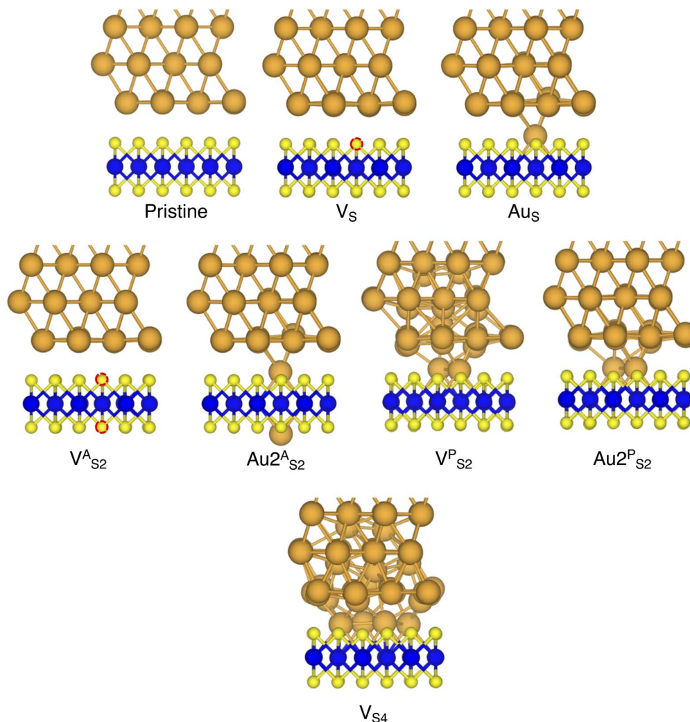
Fig. 2 Optimized geometries with DFT of selected Au/MoS 2 interfaces considered in this work. The pictures were taken in the vicinity of the contact area between the two materials. Interfaces V S2 and V S4 refer to MoS 2 with clusters of two and four S vacancies, although following geometry optimization such clusters were fully filled by Au atoms migrating from the above electrode.
