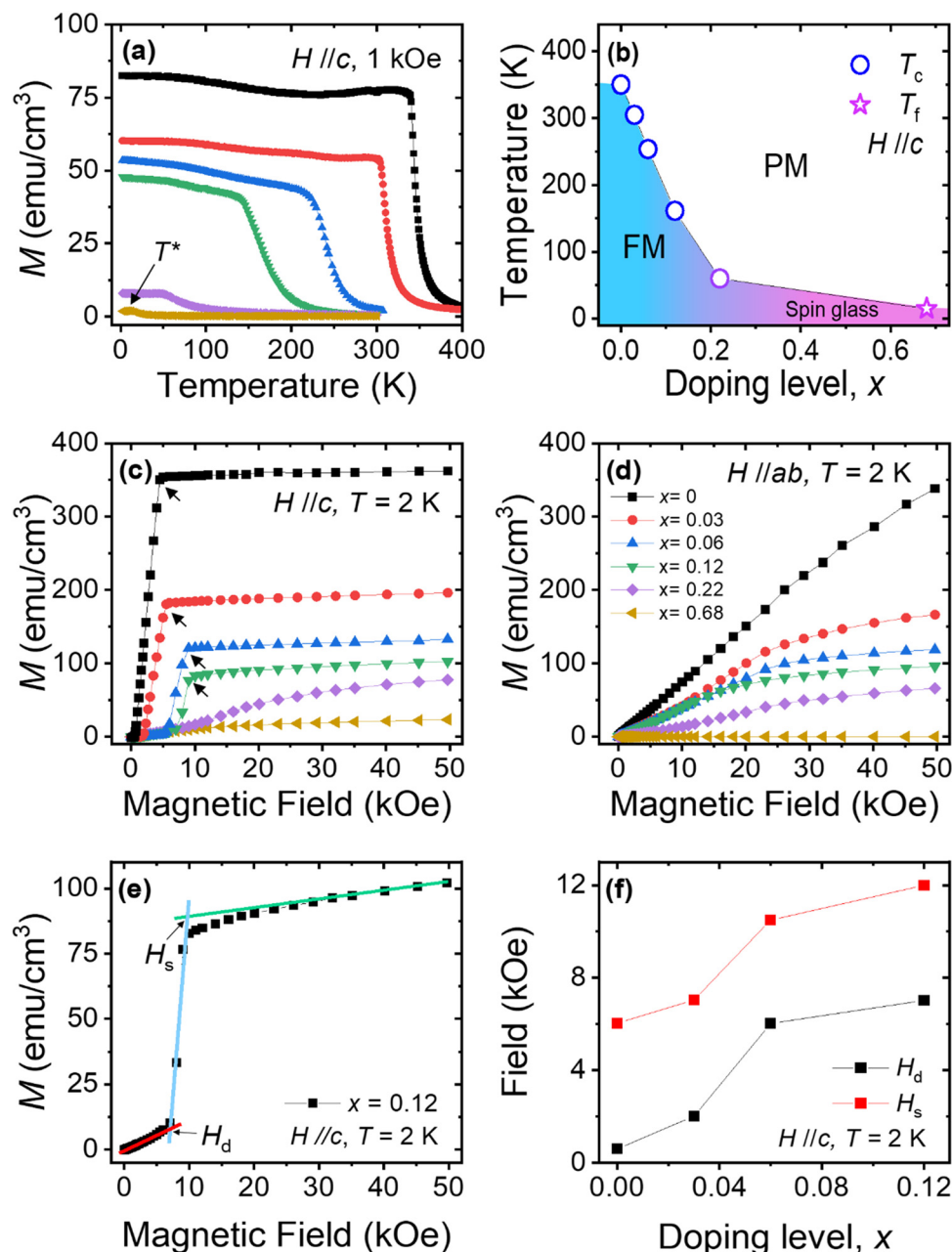
Fig. 2 Magnetic characteristics of FNGT. (a) Temperature-dependent magnetization ( M – T ) curves of FNGT with x = 0 –0.68. (b) Transition temperature of FNGT. For FNGT with x = 0 –0.22, the plotted transition temperature is the Curie temperature ( T_c ) as they show ferromagnetic (FM) characteristics. (c) Isothermal magnetization ( M – H ) curve of FNGT with H // c measured at 2 K. Arrow pointed magnetization is the saturation magnetization ( M_s ) of each crystal. (d) M – H curve of FNGT with H // ab measured at 2 K. (e) M – H curve of FNGT with x = 0.12 , H // c at 2 K. The red, blue, and green lines are linearly fitted curves in the pinning state, depinning state, and saturation state, respectively. H_d and H_s correspond to the depinning field and saturation field, respectively. (f) x dependence of H_d and H_s obtained from the M – H curves of FNGT with H // c , 2 K.
