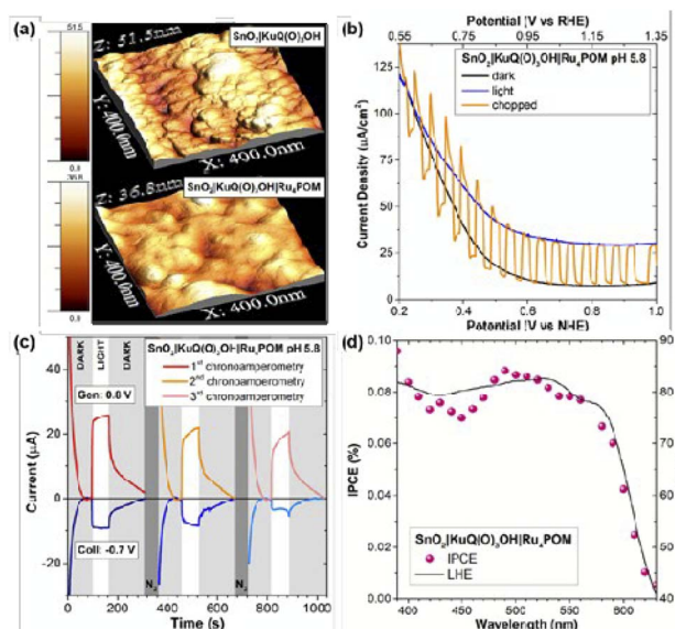
Fig. 13 (a) AFM images of KuQ 3 CO 2 H|SnO 2 and Ru 4 -POM|KuQ 3 CO 2 H|SnO 2 photoanodes. (b) Linear sweep voltammetry for Ru 4 POM|KuQ 3 CO 2 H|SnO 2 (CE: Pt; RE: Ag/AgCl 3 M NaCl; 20 mV s -1 ; light: AM 1.5G + 400 nm cut-off filter). (c) Consecutive G-C experiments for O 2 detection with Ru 4 POM|KuQ 3 CO 2 H|SnO 2 ; the positive photocurrent (red, orange, pink traces) is accompanied by a negative current of O 2 reduction at the FTO collector (blue, light blue, azure traces); CE: Pt; RE: Ag/AgCl 3 M NaCl; light: white LED + 400 nm cut-off filter. (d) IPCE (purple dots) and LHE (black line) of Ru 4 POM|KuQ 3 CO 2 H|SnO 2 . Water oxidation conditions: 0.1 M Na 2 SiF 6 /NaHCO 3 buffer at pH 5.8. Reproduced from ref. 72 with permission from the Royal Society of Chemistry.
