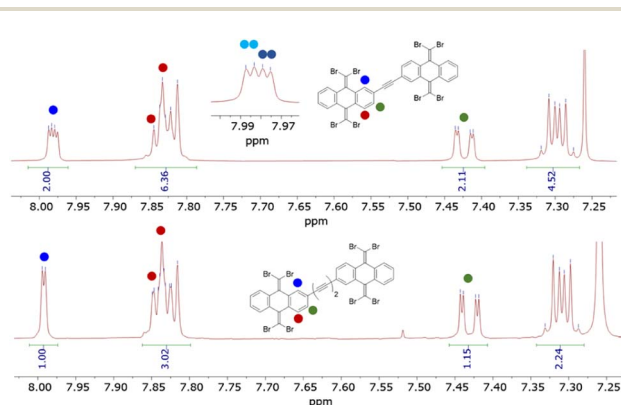
Fig. 2 Comparison of the ^1\text{H} -NMR spectra of TBQ2 and TBQ5 showing the splitting of the peri hydrogen signal of the former, consistent with the presence of two isomeric species.
