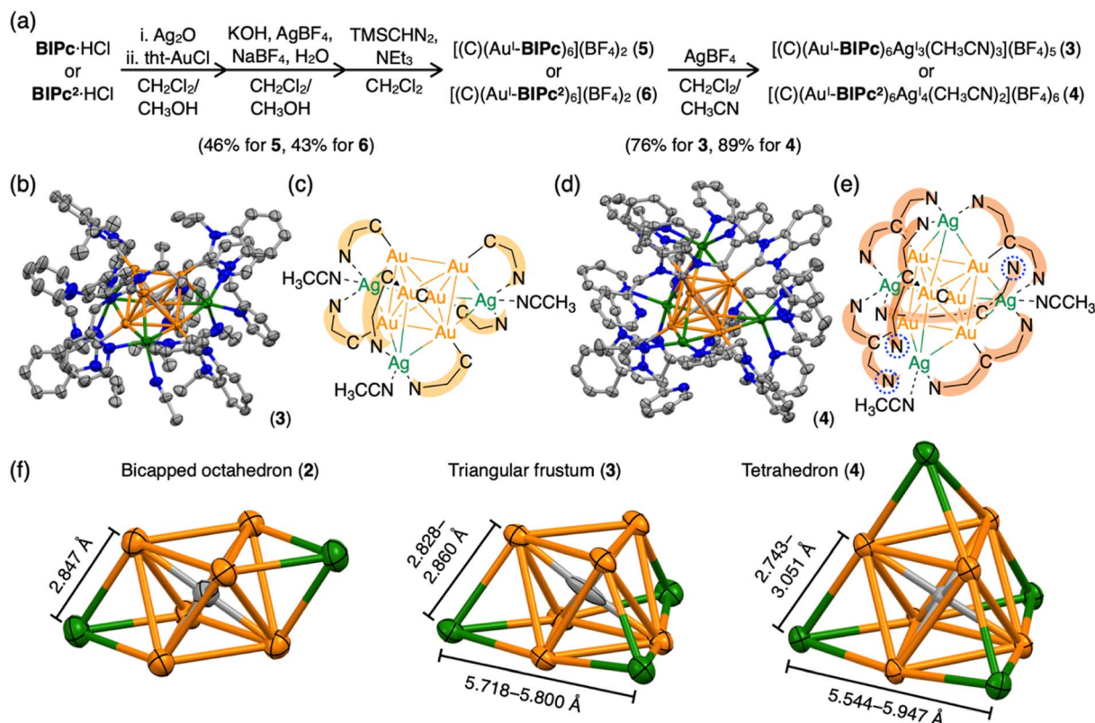
Fig. 2 (a) Synthetic schemes of the homometallic clusters [(C)(Au^I-BIPc)_6](BF_4)_2 ( 5 ) and [(C)(Au^I-BIPc)_6](BF_4)_2 ( 6 ), and heterometallic clusters [(C)(Au^I-BIPc)_6Ag_3^I(CH_3CN)_3](BF_4)_5 ( 3 ) and [(C)(Au^I-BIPc)_6Ag_4^I(CH_3CN)_2](BF_4)_6 ( 4 ). (b) Molecular structure of cluster 3 . (c) A simplified scheme showing the structure of cluster 3 . C ∧ N represents ligand BIPc . (d) Molecular structure of cluster 4 . (e) A simplified scheme showing the structure of cluster 4 . N ∧ C ∧ N represents ligand BIPc 2 . Uncoordinated pyridyl groups are highlighted by dashed blue cycles. (f) Comparison of structures of bicapped octahedral CAu_6Ag_2 in cluster 2 , triangular frustum-shaped CAu_6Ag_3 in cluster 3 , and tetrahedral CAu_6Ag_4 in cluster 4 . The length of the edge of each structure is shown.
