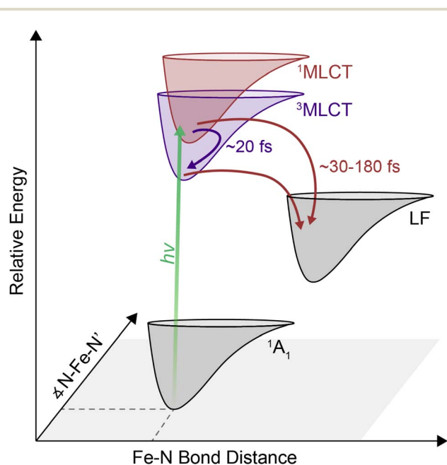
Fig. 6 Proposed energy relaxation diagram derived from 2DES experiments. The initially-excited MLCT states relax into a lower-lying excited ligand field (LF) state at a solvent-dependent timescale. The timescales denoted represent the range reported in this study. Singlet-to-triplet intersystem crossing within the MLCT manifold occurs simultaneously on a timescale of \sim 10\text{--}20\text{ fs} .
