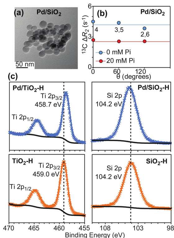
Fig. 7 Properties of Pd/SiO 2 . Panel (a) shows a TEM image for the investigated Pd/SiO 2 material. Panel (b) shows a plot of the 13 C Δ R 2 as a function of \theta measured for PhOH in the presence of 1 wt% Pd/SiO 2 . The ortho (2.6) and meta (3.5) positions generate equivalent NMR peaks and one single Δ R 2 value for these peaks is reported. Data measured in the presence of 0 and 20 mM Pi are shown as blue and red spheres, respectively. Solid blue and red lines are the corresponding average Δ R 2 values. Panel (c) shows XPS spectra measured for TiO 2 (bottom left), Pd/TiO 2 (top left), SiO 2 (bottom right), and Pd/SiO 2 (top right) after hydrogen treatment (see ESI Methods†). The shift of the XPS Ti 2p peaks after hydrogen treatment is consistent with Ti reduction in the presence of supported Pd.
