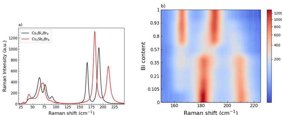
Fig. 4 (a) Comparison between room temperature (RT) Raman spectra of the end-members. (b) Color map reporting the modes intensity of the sample spectra in the range between 150 and 225 cm -1 as a function of Bi content (we applied a power-law normalization to remap the colors, to increase the contrast and better point out the change in the mode position).
