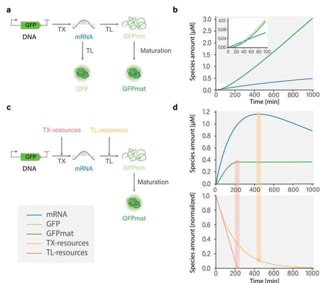
Fig. 2 Influence of model composition on simulated dynamics of cell-free GFP expression in the PURE system; (a) structure of model developed by Karzbrun 26 that includes TXTL reactions with and without protein maturation processes; (b) simulated dynamics of the model developed by Karzbrun. 26 Simulation of GFP expression dynamics shows that incorporation of protein maturation processes results in delayed appearance of detectable GFP. Protein and mRNA synthesis do not reach a steady state due to the absence of resource use reactions that limit synthesis. (c) Structure of model developed by Stögbauer 14 that includes TXTL, resource use, and protein maturation reactions; (d) simulated dynamics of the model developed by Stögbauer. 14 Protein synthesis reaches a steady state coinciding with the depletion of translational resources (TL-resources), as indicated by the red rectangular highlight. Notably, overall mRNA concentration decreases over time, even in the presence of available transcriptional resources (TX-resources), as indicated by the yellow rectangular. This underscores the importance of providing a more comprehensive description of resource use.
