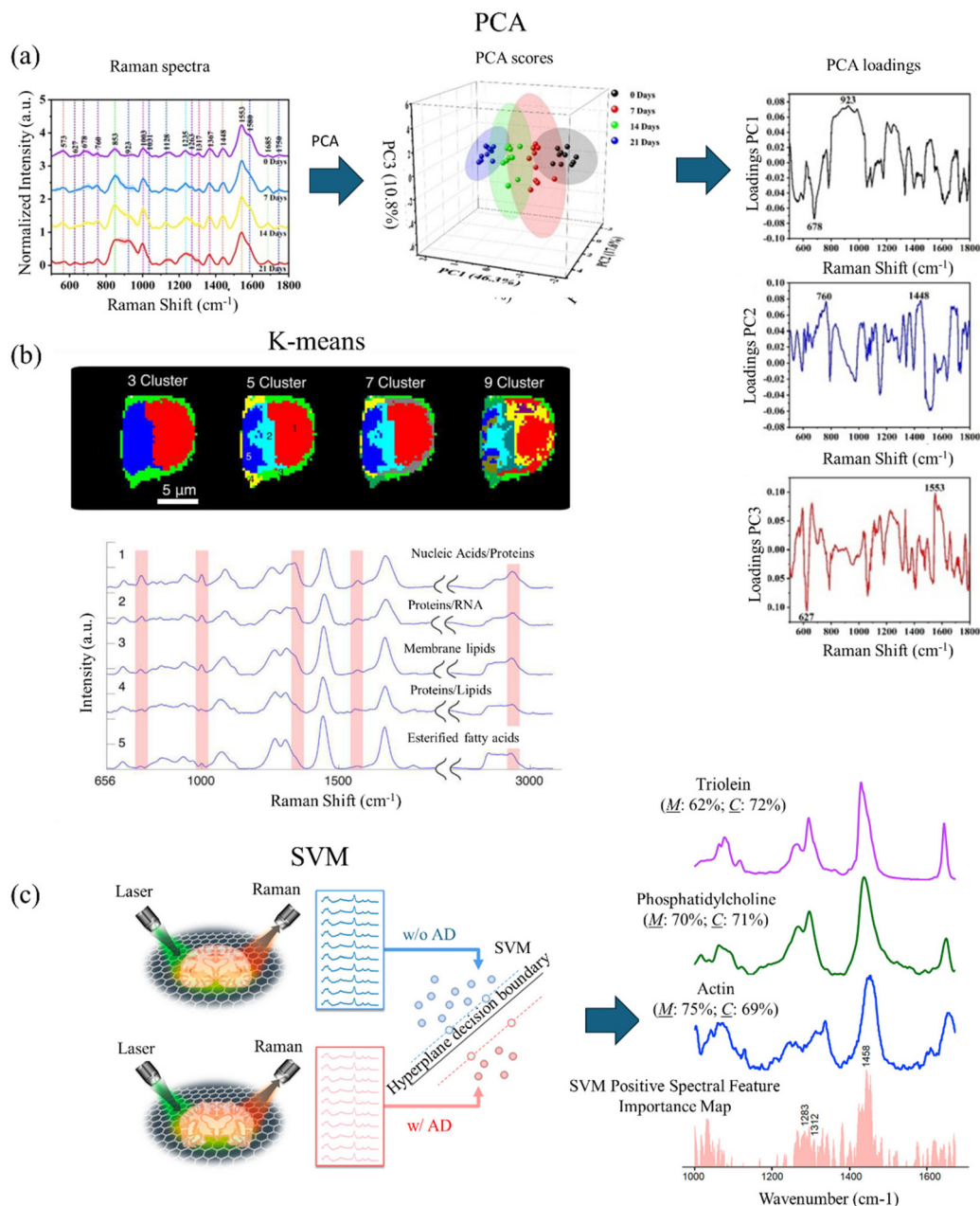
Fig. 3 (a) Using PCA to analyze SERS spectra measured from AD mice serum at different stages. PCA score plot for SERS measured spectra of AD mice serum at different stages. PCA loading plot for first three principal components. Adapted with permission from ref. 119. Copyright 2023 Elsevier. (b) K-means cluster-based Raman mapping of lymphocyte cells with different numbers of clusters. Mean spectra of clusters with the number of clusters equal to 5. Adapted with permission from ref. 121. Copyright 2013 SAGE Publications. (c) Using SVM to classify Raman spectra measured from mice brain samples with and without AD. Linear SVM trained, which classifies the brain samples with and without AD using a hyperplane decision boundary. The spectral feature importance obtained from SVM and Raman spectra of potential biomarkers of AD. Adapted with permission from ref. 23. Copyright 2022 American Chemical Society.
