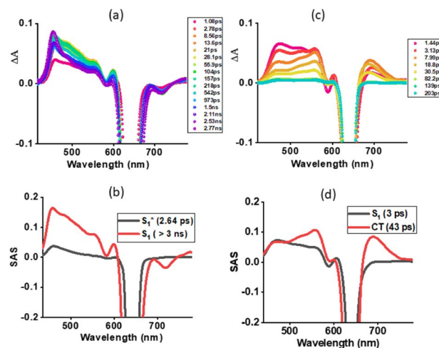
Fig. 7 Femtosecond transient absorption spectra at the indicated delay times of (a) 1 and (c) 2 in DMSO ( \lambda_{ex} = 648 nm). Species associated spectrum from GloTarAn analysis is shown beneath for each spectrum.
