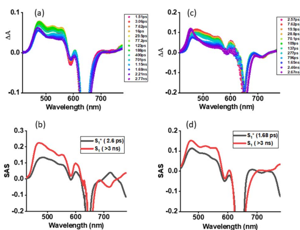
Fig. 6 Femtosecond transient absorption spectra at the indicated delay times of (a) 1 and (c) 2 in toluene ( \lambda_{ex} = 648 nm). Species associated spectrum from GloTarAn analysis is shown beneath for each spectrum.
