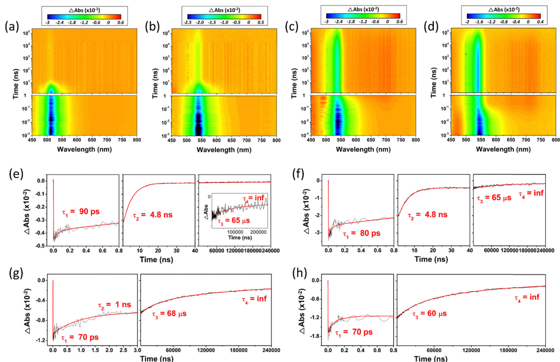
Fig. 7 fs-to- \mu\text{s} TA 2D map of (a) PY-BDP, (b) PY-BDP-2Cl, (c) PY-BDP-2Br, and (d) PY-BDP-2I in toluene under photoexcitation at 500 nm. TA decay profiles of (e) PY-BDP, (f) PY-BDP-2Cl, (g) PY-BDP-2Br, and (h) PY-BDP-2I at 505, 535, 535, and 540 nm, respectively. Because our measured time window, 240 \mu\text{s} , is not enough to measure the longest decay time constant, we estimated the other time constants with the last infinite time constant.
