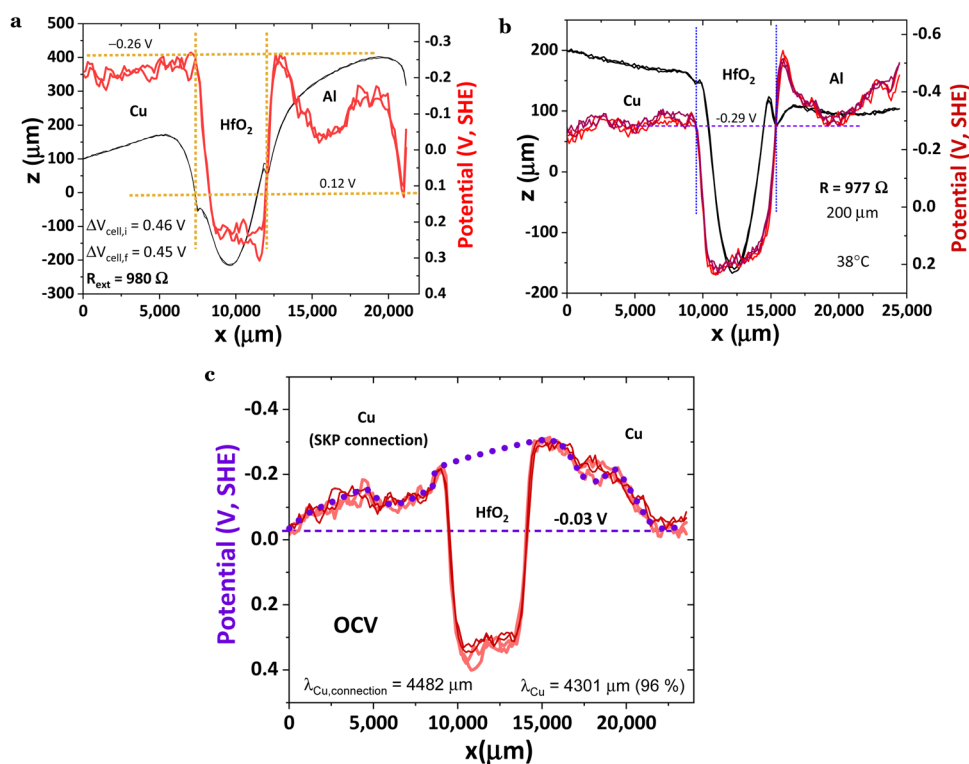
Fig. 6 Surface chemical potentials for Cu/ \text{HfO}_2 /Al cells in a closed circuit while connected to a resistor load of \sim 980 \Omega ; (a) showing equalization of the surface chemical potentials for Cu/ \text{HfO}_2 with Al at -0.26 V and \text{HfO}_2/\text{Al} with Al at 0.12 V with the SKP probe tip positioned 150 \mu\text{m} from the cell during the analyses; (b) showing equalization of the surface chemical potentials for Cu/ \text{HfO}_2 with \text{HfO}_2/\text{Al} and Al with the SKP probe positioned 200 \mu\text{m} away from the cell during the analyses; (c) symmetric Cu/ \text{HfO}_2 /Cu cell at OCV showing equalization of the chemical potentials at Cu ( 0 \mu\text{m} ), Cu/ \text{HfO}_2 , \text{HfO}_2/\text{Cu} , and Cu ( 22.5 \text{ mm} ) at -0.03 V with the plasmonic waves incident and transmitted in both Cu(s) being not attenuated or suffering a small attenuation through the \text{HfO}_2 , which performs as a connection between both coppers, the first Cu connected to the SKP and the second Cu in electrical contact with the first through the \text{HfO}_2 . The wavelength of the plasmonic waves on the surface of the Cu connected to the SKP is \lambda_{\text{Cu,connection/air}} = 4482 \mu\text{m} , and in the remaining Cu is \lambda_{\text{Cu/air}} = 4301 \mu\text{m} , corresponding to 96% of the wavelength of the Cu connected to the SKP.
