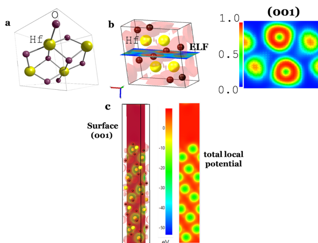
Fig. 2 Structure of hafnium oxide (monoclinic phase P 2 1 / c ): (a) crystalline structure; (b) electron localization function (ELF) of a (001) slice; ELF = 1 and ELF = 1/2 corresponding to the localized and electron gas; (c) total local potential of a surface (001) of HfO 2 .
