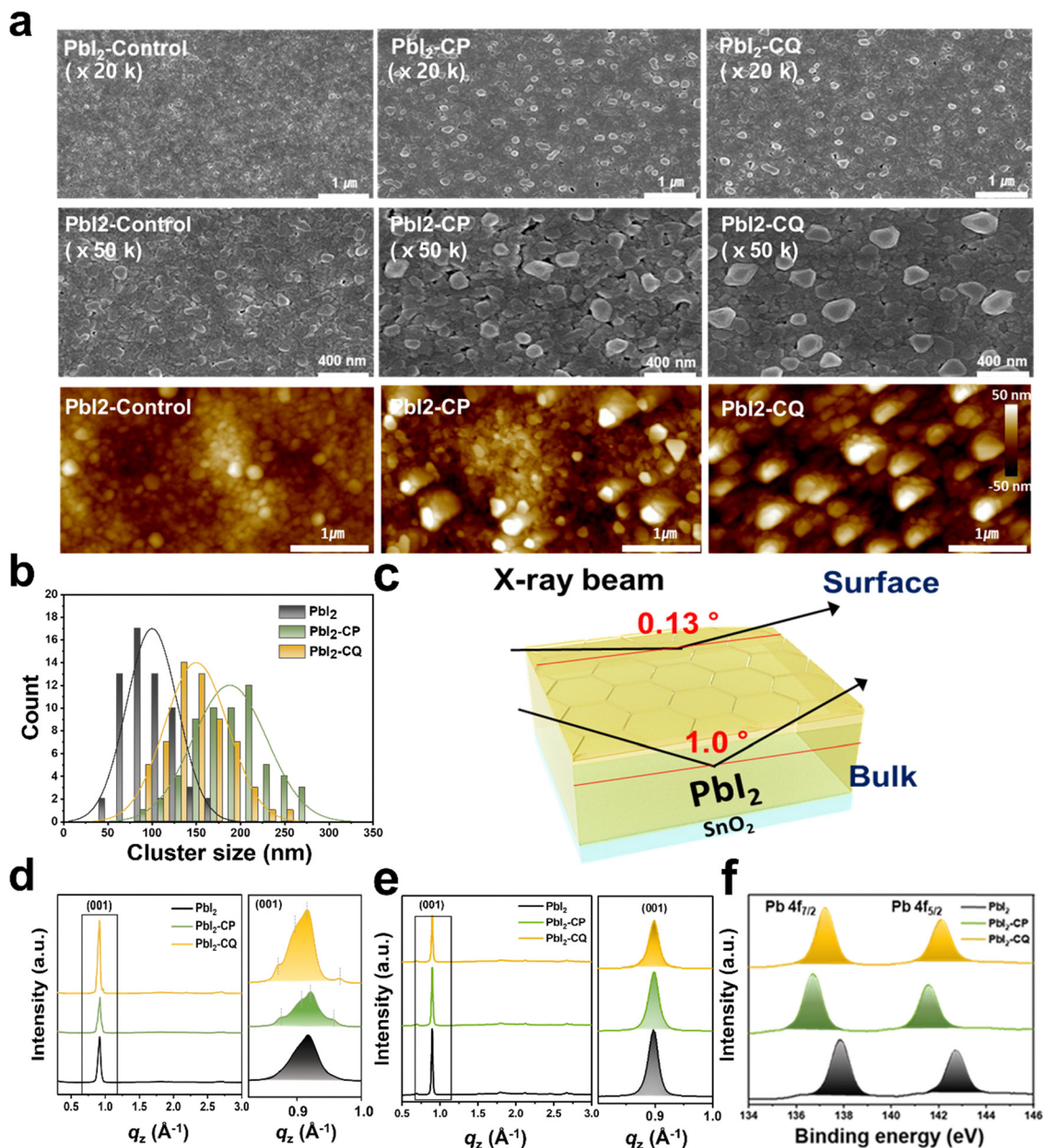
Fig. 3 Effect of CP and CQ additives on PbI 2 film morphology. (a) Top-view SEM images of PbI 2 -control, CP, and CQ with AFM images of the inset (4 \mu m \times 4 \mu m). (b) Cluster size distribution of pristine PbI 2 , PbI 2 -CP, and PbI 2 -CQ. (c) Schematic illustration of the angle-dependent 2D-GIWAXS measurement. Line-cut profile of PbI 2 (001) of the control, CP-, and CQ-PbI 2 for (d) 0.13^\circ and (e) 1.0^\circ incident angles. (f) XPS spectra (Pb 4f) of PbI 2 pristine, PbI 2 -CP, and PbI 2 -CQ.
