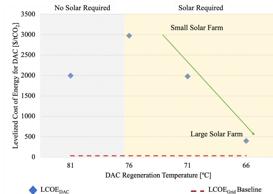
Fig. 8 Levelized cost of energy for DAC delivered by the DAC in series – upstream configuration using a low-temperature geothermal reservoir, compared to the baseline leveled cost of the grid electricity generation baseline case.
