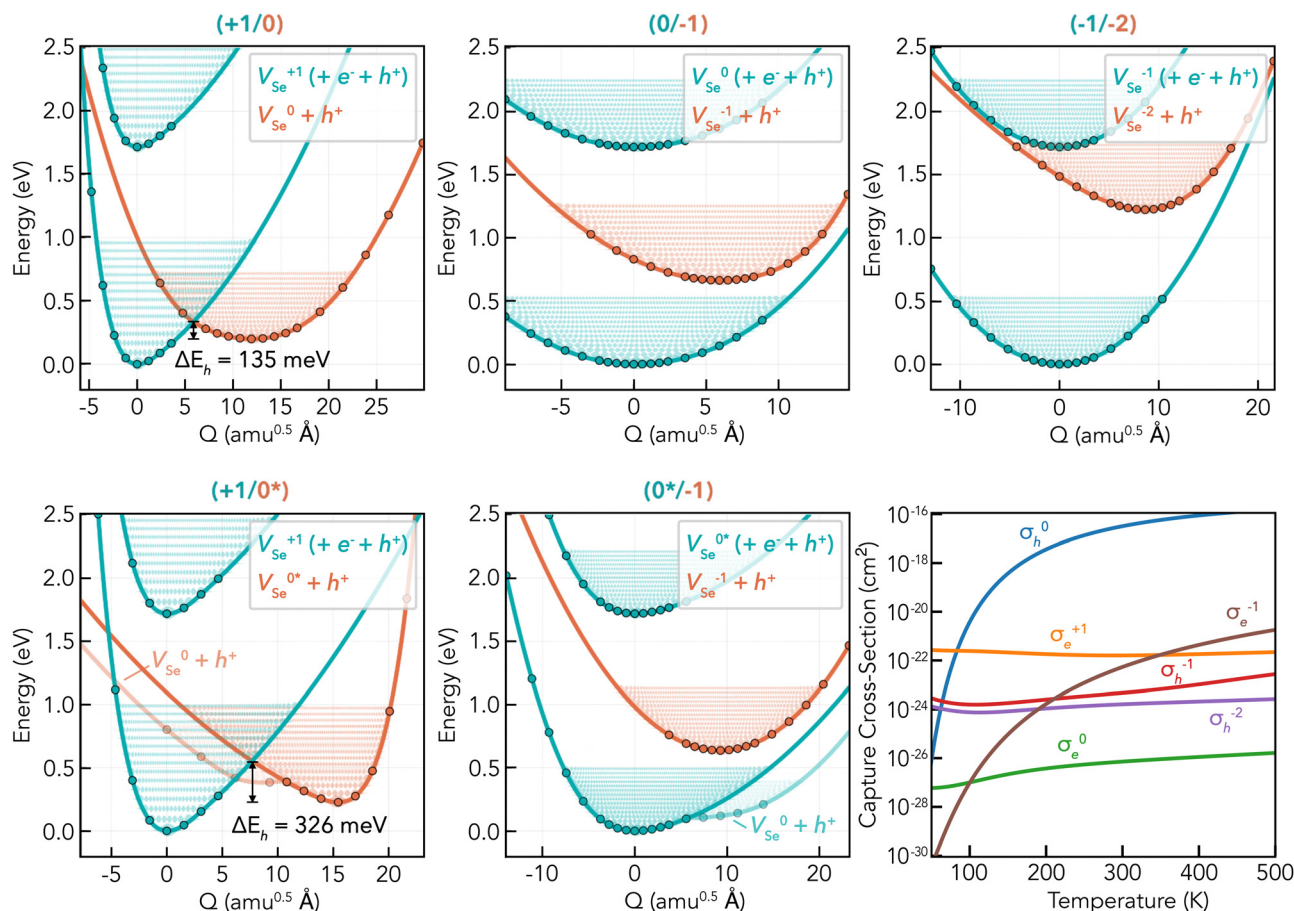
Fig. 6 Potential energy surfaces (PES) and corresponding charge capture cross-sections of vacancy defects in t-Se. Each plot shows V_{\text{Se}} PES in two charge states; X^q in blue, X^{q-1} + h^+ in orange, and X^q again with an electron–hole pair of energy equal to the band gap E_g (upper blue PES); along the linear path in structural space between their equilibrium configurations, with the corresponding defect level given as the plot title ( q/q-1 ). The transition from the upper blue ( X^q + e^- + h^+ ) to middle orange ( X^{q-1} + h^+ ) PES corresponds to electron capture by X^q , while that from middle orange to lower blue ( X^q ) corresponds to hole capture by X^{q-1} . The x-axis corresponds to the structural/configurational coordinate Q , given in units of mass-weighted displacement (Ångstrom times the square root of the atomic mass unit; amu 0.5 Å). \Delta E_{h/e} denotes the activation energy barrier to hole/electron capture, here for the two cases which show a crossing between PES and thus a classical capture barrier. Filled circles represent calculated energies, and the solid lines are spline fits to the data. A portion of the effective vibrational wave functions are also shown for illustration. In the bottom-right plot, the corresponding charge capture cross-sections of each vacancy defect level are plotted as a function of temperature. The charge of the defect is given by the superscript, and the charge carrier is denoted by the subscript; e/h for electron/hole; \sigma_{e/h}^0 . For transitions involving the neutral state, the faster of the V_{\text{Se}}^0/V_{\text{Se}}^{0*} rates are shown; which is V_{\text{Se}}^0 in all cases except for \sigma_e^0 – which is extremely slow in both cases. The charge capture coefficients are plotted in Fig. S11 (ESI†).
