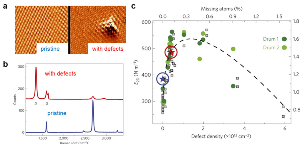
Fig. 12 Experimental understanding of a defect's impact on elastic modulus. (a) Atomic-resolution scanning tunnelling microscopy (STM) characterization of a pristine graphene, before Ar + irradiation (left panel), and after irradiation, which shows a single defect containing a vacancy cluster (right panel). 134 (b) Raman spectra taken from the sample before and after the irradiation treatment, denoted by blue and red colours respectively. The intensity ratio between the D and G peaks can be used to evaluate to defect density. 134 (c) E_{2D} measured by AFM nanoindentation as a function of defect concentration. Reproduced from ref. 134 with permissions from Springer Nature Limited Copyright 2014. 134
