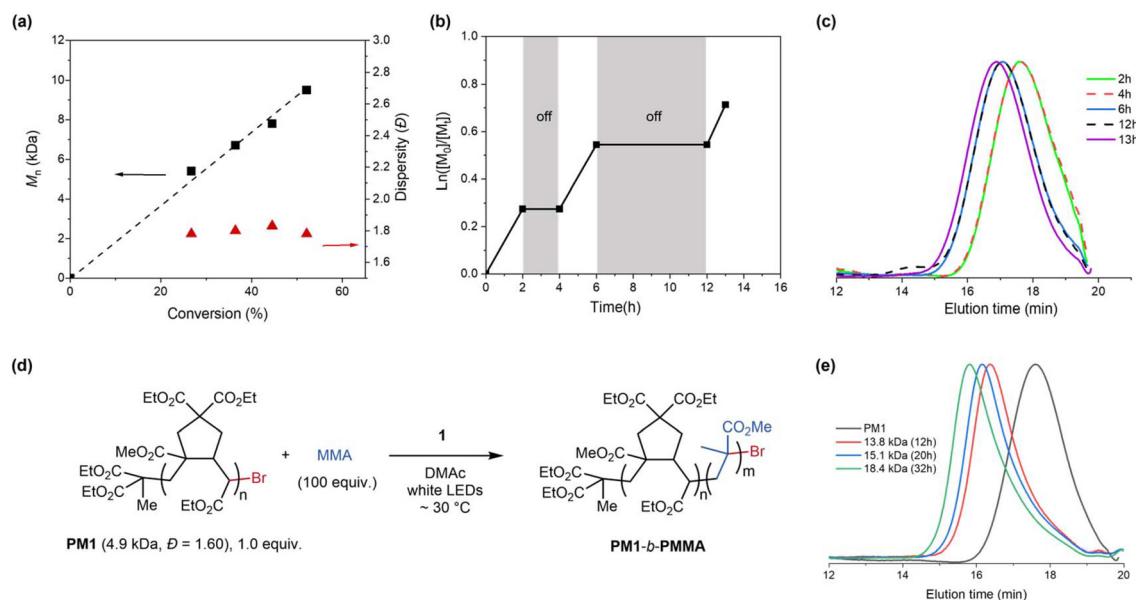
Fig. 4 (a) Plots of measured M_n and \bar{D} as a function of monomer conversion for polymerization of [M1]/[DBMM]/[PC1] = 500/10/1 performed in PhCl (0.5 M), at ~30 °C, with 1.4 W white LED irradiation. (b) Plots of natural log of monomer conversion as a function of time and (c) overlaid GPC traces for the pulsed irradiation experiment. (d) Chain-extension polymerization from a PM1 macroinitiator with MMA. (e) Overlaid GPC traces for chain-extension polymerization.
