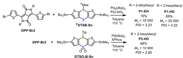
Scheme 1 Synthetic scheme of DTSB/DTSO 2 B-containing polymers.
