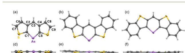
Fig. 2 ORTEP of (a and d) 3a , (b and e) 3c , and (c and f) 3d . Thermal ellipsoids are drawn at the 50% probability level.
