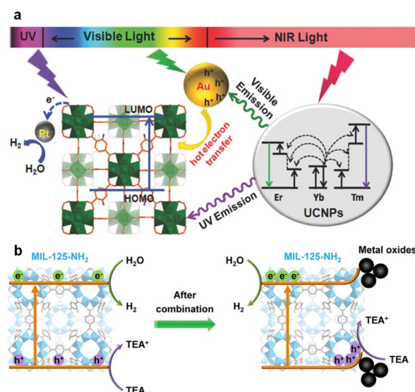
Fig. 10 (a) The light absorption region of \text{UCNPs-Pt@MOF/Au} . 87 Copyright 2018, John Wiley and Sons. (b) Schematic diagram of photocatalytic hydrogen production over \text{MIL-125-NH}_2 and metal oxides/ \text{MIL-125-NH}_2 . 93 Copyright 2022, John Wiley and Sons.
