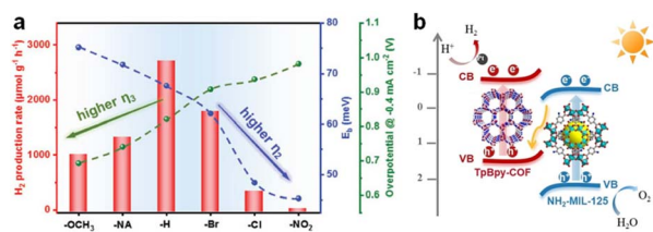
Fig. 9 (a) Photocatalytic \text{H}_2 production rate, E_b and overpotential in the HER of \text{UiO-66-NH}_2\text{@Pt@UiO-66-X} . 82 Copyright 2023, John Wiley and Sons. (b) Photocatalytic mechanism of the S-scheme heterojunction in \text{NH}_2\text{-MIL-125/TpBpy-COF} for overall water splitting. 84 Copyright 2025, John Wiley and Sons.
