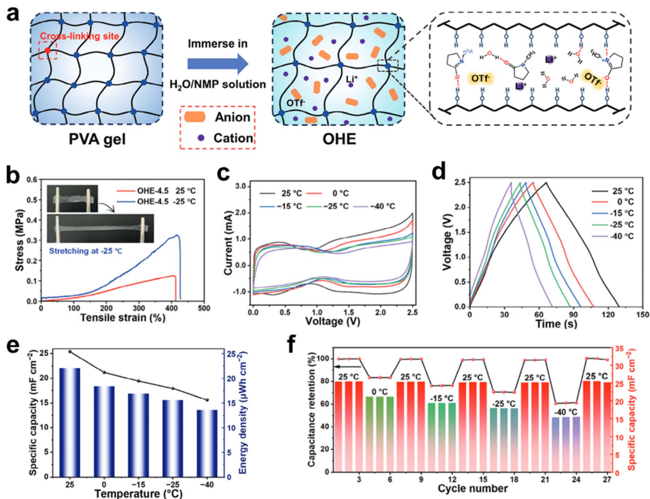
Fig. 10 Anti-freezing hydrogel electrolytes designed by introducing organic solvents. (a) Preparation process of the gel electrolyte. (b) Tensile stress–strain curves at 25 and -25^\circ\text{C} of the gel electrolyte. (c) CV curves and (d) GCD profiles of supercapacitors from 25 to -40^\circ\text{C} . (e) Specific capacitance and energy density of supercapacitors at different temperatures. (f) Continuous reversible changes of capacitance retention of supercapacitors under various temperature conditions. Reproduced with permission. 56 Copyright 2025, Wiley-VCH.
