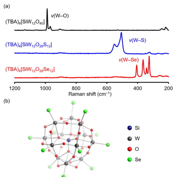
Fig. 3 (a) Raman spectra of (\text{TBA})_4[\text{SiW}_{12}\text{O}_{40}] (black), (\text{TBA})_4[\text{SiW}_{12}\text{O}_{28}\text{S}_{12}] (blue), and (\text{TBA})_4[\text{SiW}_{12}\text{O}_{28}\text{Se}_{12}] (red). (b) Crystal structure of the anionic component of the tetraphenylphosphonium (TPP) salts of [\text{SiW}_{12}\text{O}_{28}\text{Se}_{12}]^{4-} . Color code: dark blue, Si; black, W; red, O; light green, Se.
