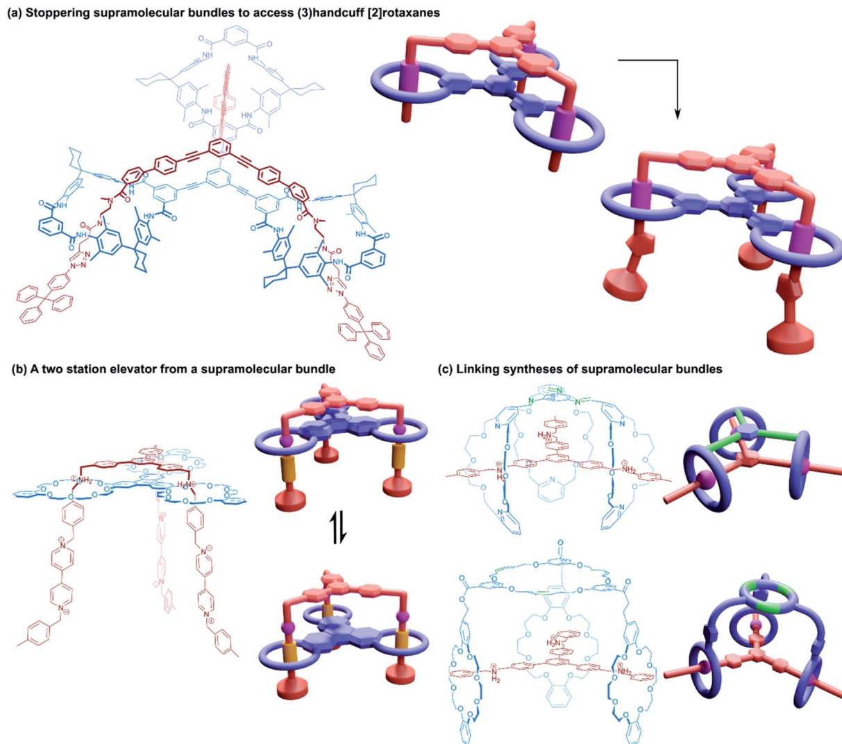
Fig. 11 (3)Handcuff [2]rotaxanes. (a) The stoppering of a supramolecular bundle made from a tris(tetralactam) host via azide–alkyne cycloaddition to give a (3)handcuff [2]rotaxane; (b) a two station molecular elevator with a platform that moves between viologen and dibenzylammonium stations; (c) linking synthesis of supramolecular bundles using olefin metathesis and imine formation.
