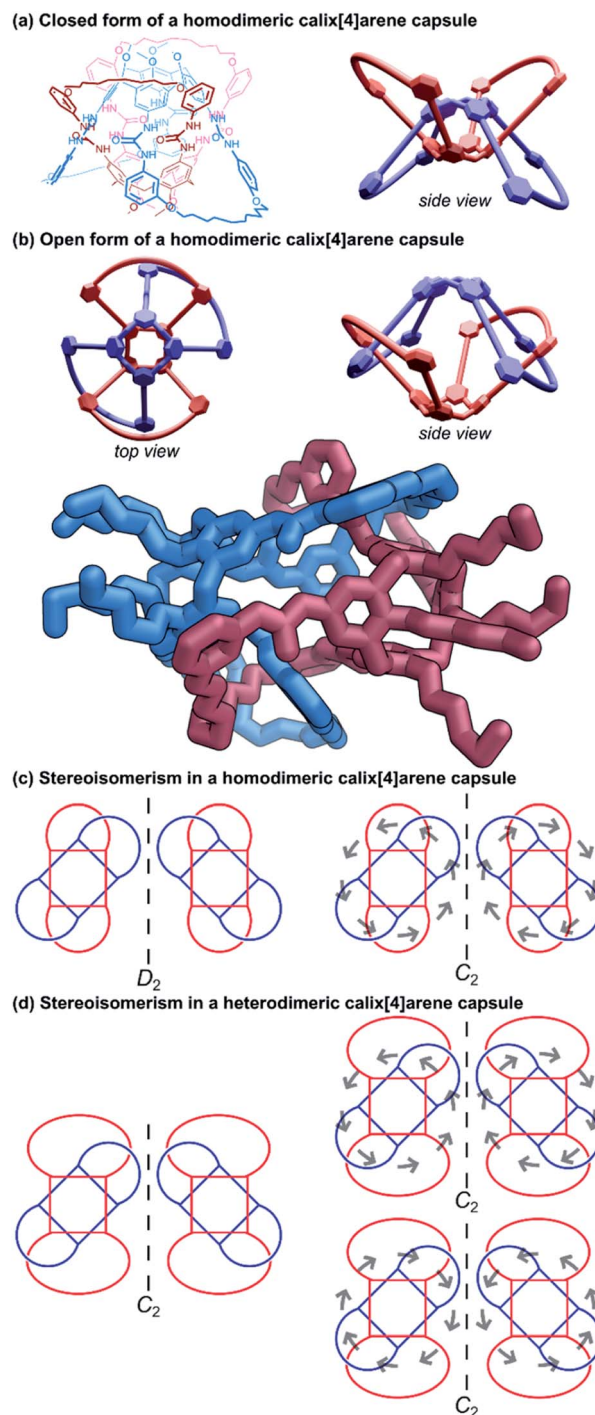
Fig. 10 Cyclic (2)handcuff [2]catenanes synthesised via dimeric calix [4]arene capsules. (a) Chemical structure and schematic representation of such a handcuff in the closed form; (b) schematic representations and a crystal structure representation of the open form. Hydrogen atoms have been omitted on the representation of the single crystal X-ray structure; (c) stereoisomerism possible in a homodimeric handcuff capsule, with grey arrows indicating the direction of the hydrogen bonding in the urea belt; (d) stereoisomerism possible in a heterodimeric handcuff capsule, with grey arrows indicating the direction of the hydrogen bonding in the urea belt.
