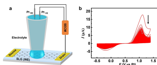
Fig. 1 (a) Schematic diagram of SLG bromination process. (b) Cyclic voltammograms of SLG microstrip electrode in an aqueous solution with 10 mM KBr and 10 mM H_2SO_4 ; the scan rate is 100 mV s^{-1} .
