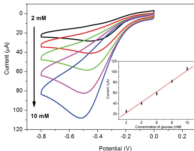
Fig. 5 Cyclic voltammograms of chitosan/GOD/AgNPs-G/GCE in O 2 saturated 0.2 M PBS at pH 7.4 in various concentrations of glucose. Inset is the calibration curves corresponding to amperometric responses at -0.5 V.
