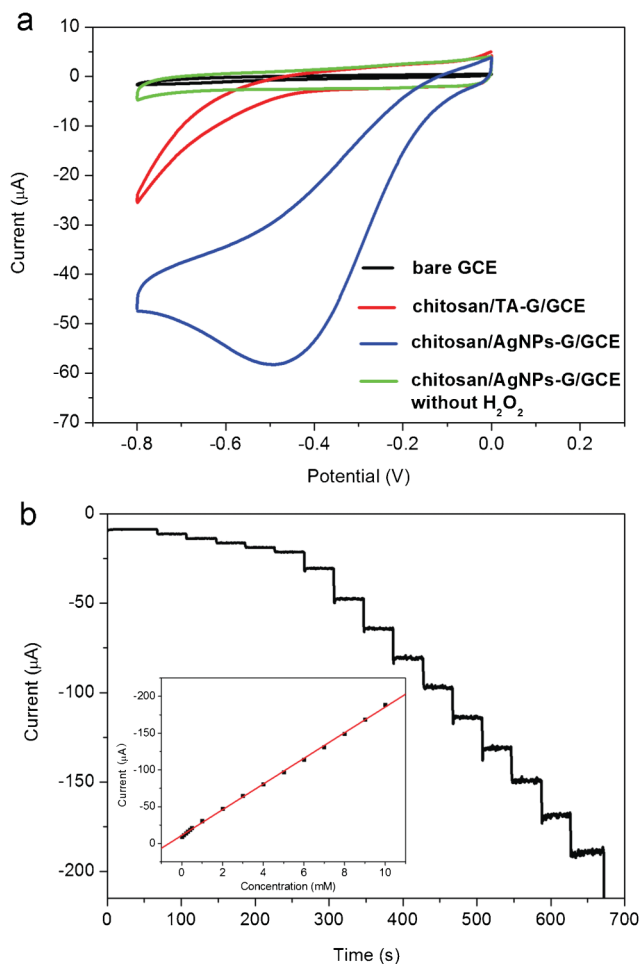
Fig. 4 (a) Cyclic voltammograms of different electrodes in N 2 -saturated 0.2 M PBS at pH = 7.4 in the presence of 2 mM H 2 O 2 (scan rate: 50 \text{mV s}^{-1} ). (b) Typical steady-state response of the chitosan/AgNPs-G/GCE to successive injection of H 2 O 2 into the stirred N 2 -saturated 0.2 M PBS at pH = 7.4. Inset: the corresponding calibration curve (Applied potential: -0.3 V).
