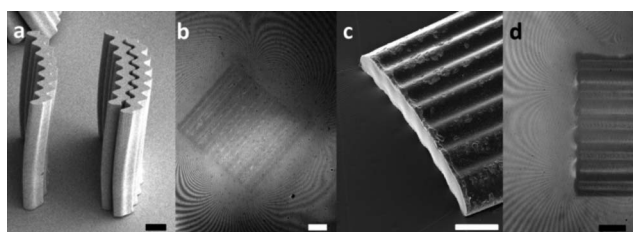
Fig. 3 (a) SEM image (JEOL 7500F HRSEM) of the microstructures. (b) Interference fringes around such a microstructure in isolation at the air–water interface clearly show the four-lobed quadrupolar deformation of the interface. (c) SEM and (d) microinterferometry of the interface undulations near the ends of a microstructure. The scale bars correspond to 50 \mu\text{m} .
