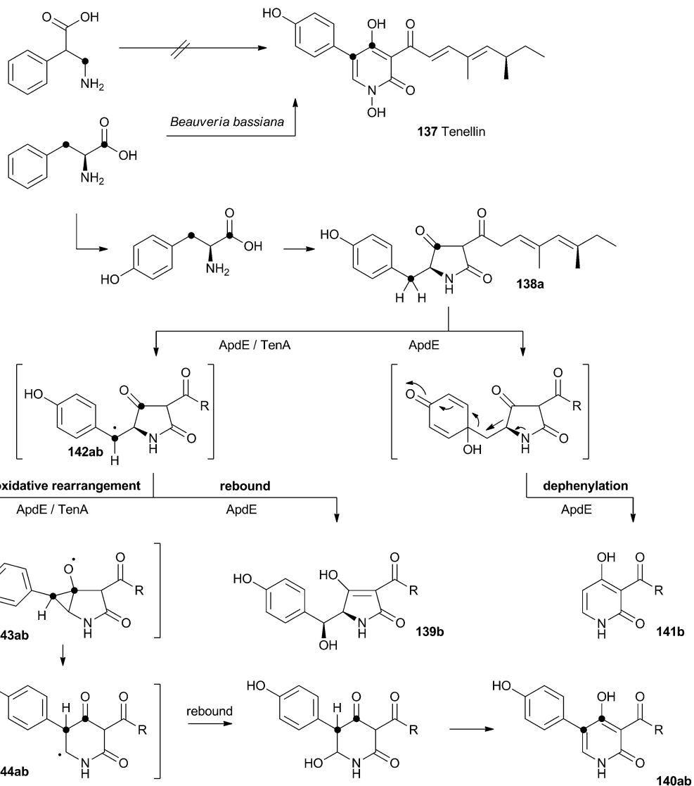
Scheme 22 Oxidative rearrangements during the biosynthesis of 2-pyridones. (a) (Tenellin) series: R = CHCHC(Me)CHCH(Me)CH 2 Me; (b) (aspyridone) series R = CH(Me)CH 2 CH(Me)CH 2 Me.
