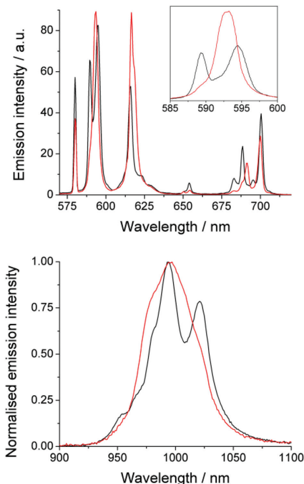
Fig. 1 Change in form of emission spectra with fluoride. Top: EuDTMA in D 2 O (black) and with excess sodium fluoride (red), \lambda_{ex} = 394 nm, exit slit = 1 nm; inset shows the change in structure of the \Delta J = 1 band measured with 0.2 nm exit slit. Bottom: YbDTMA in D 2 O (black) and with added fluoride (red), \lambda_{ex} = 265 nm, exit slit = 5 nm.
