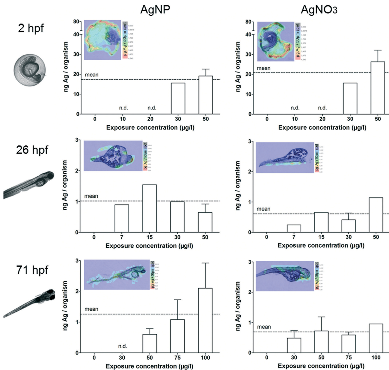
Fig. 3 Silver concentrations measured for ZFE exposed at different developmental stages (2, 26, and 71 hpf) in the presence of sublethal effects. Quantification results obtained by neb-ICP-MS and respective LA-ICP-MS images after 24 h of exposure are shown. The color scale bar of the LA-ICP-MS measurements represents silver concentrations from the highest (red) to the lowest value (blue). The table below shows the calculated means over the exposure concentrations (dotted line in graphs).
