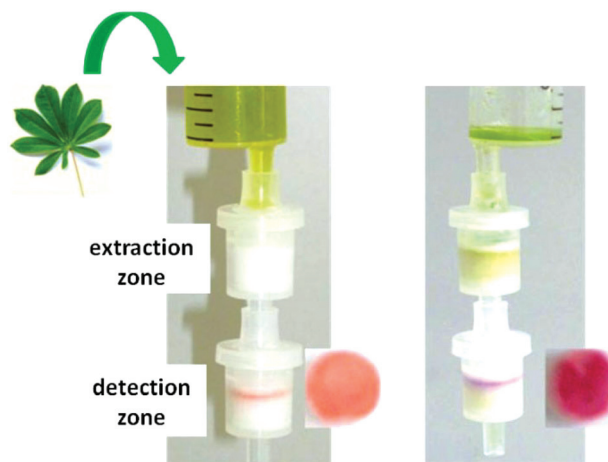
Scheme 3 Experimental setup for the detection of cyanide in a raw green-coloured extract of a cassava leaf using extraction and detection zones (adapted from ref. 20). 20
