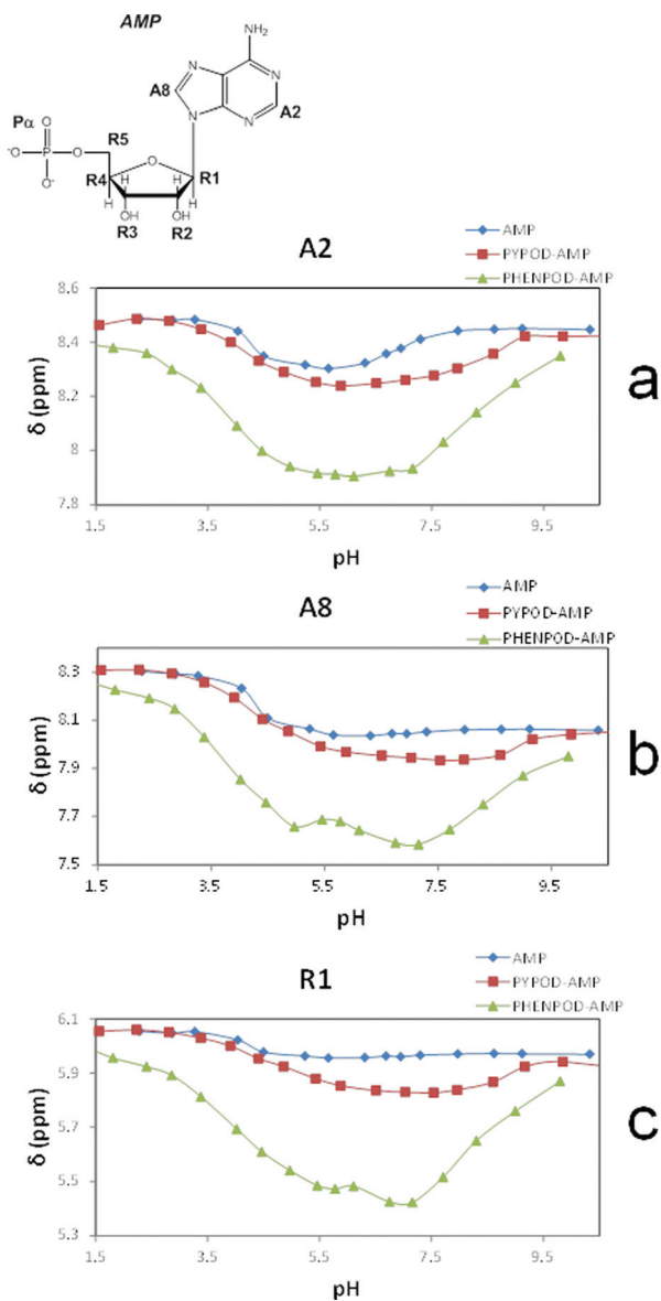
Fig. 6 ^1\text{H} NMR titration of PHENPOD (up) and PYPOD (down) with AMP, pD 6.8. For atom labelling see Scheme 1 and Fig. 5.
