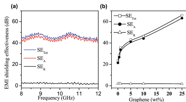
Fig. 3 (a) The comparison between SE_{\text{Tot}} , SE_{\text{R}} and SE_{\text{A}} for the graphene/PEDOT:PSS sample with 10% graphene loading, and (b) the same for samples with different graphene loadings at 10 GHz.
