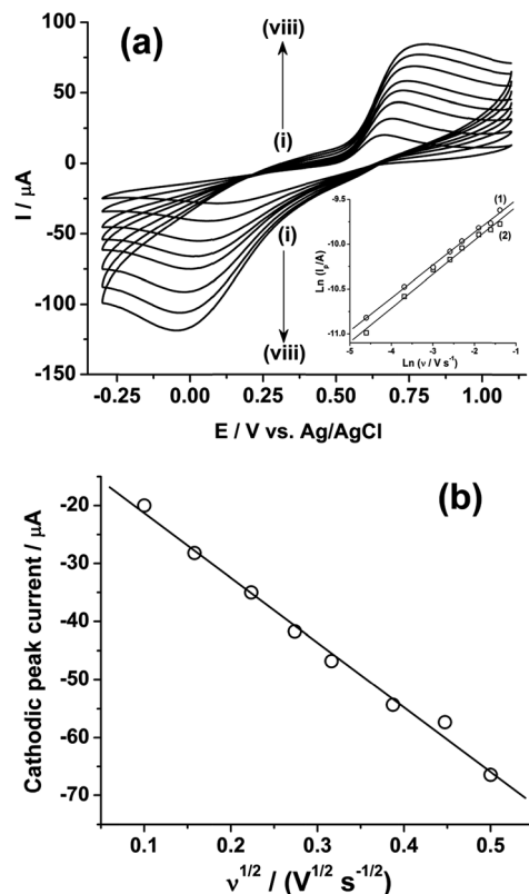
Fig. 2 (a) Cyclic voltammograms of 10 mM Pu(IV) in 1 M H 2 SO 4 solution on GC electrode at a scan rate ( v ) of (i) 10, (ii) 25, (iii) 50, (iv) 75, (v) 100, (vi) 150, (vii) 200 and (viii) 250 mV s -1 . The inset shows the plots of \ln(I_p) versus \ln(v) for (1) cathodic and (2) anodic peaks. (b) Plot of the cathodic peak current versus the square root of the scan rate ( v^{1/2} ).
