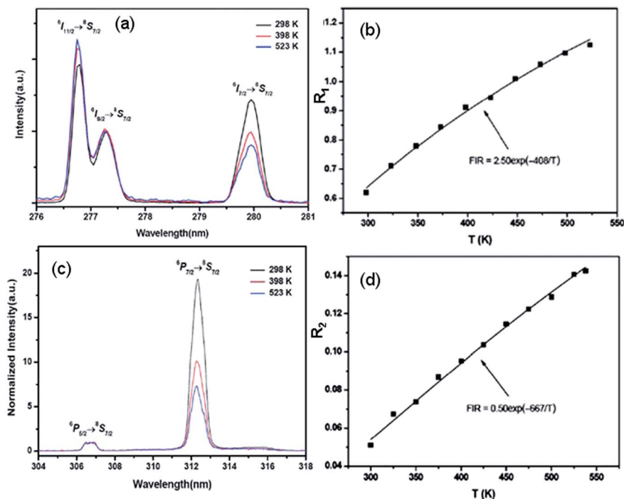
Fig. 7 Temperature dependent (a) ultraviolet spectra in the range of 276–281 nm, and (b) R_1 of the emissions from the transitions of {}^6I_{9/2}/{}^8S_{7/2} and {}^6I_{7/2}/{}^8S_{7/2} of NaLuF 4 :Yb 3+ , Tm 3+ , Gd 3+ microcrystals. Temperature dependent (c) ultraviolet spectra in the range of 304–318 nm, and (d) R_2 of the emissions from the transitions of {}^6P_{5/2}/{}^8S_{7/2} and {}^6P_{7/2}/{}^8S_{7/2} of NaLuF 4 :Yb 3+ , Tm 3+ , Gd 3+ microcrystals. Reproduced from ref. 60 with permission of the Royal Society of Chemistry.
