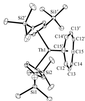
Fig. 4 Molecular structure of \text{Cp}_2\text{Th}(\text{C}_8\text{H}_8) , 4. Thermal ellipsoids are drawn at the 50% probability level and hydrogen atoms are omitted for clarity. \text{Th}\text{--C}(\text{C}_8\text{H}_8) distances ( \text{\AA} ): \text{Th}\text{--C12} , 2.815(4) ; \text{Th}\text{--C13} , 2.841(4) ; \text{Th}\text{--C14} , 2.769(3) ; \text{Th}\text{--C15} , 2.736(4) .
