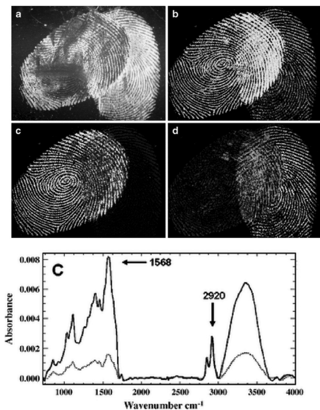
Fig. 1 (a) Cyanoacrylate-developed latent fingerprints that are superimposed. (b) Infrared absorbance distribution using the CH stretching mode at nearly 2940 \text{ cm}^{-1} . (c) The carbonyl band shown at nearly 1730 \text{ cm}^{-1} . (d) The ratio of the carbonyl band at nearly 1730 \text{ cm}^{-1} and the amide band at nearly 1640 \text{ cm}^{-1} . (e) Examples of spectra using different vibrational modes from the oil-rich region (top, dark line) and flake rich region. 22 Reproduced from ref. 22 with permission from Springer.
