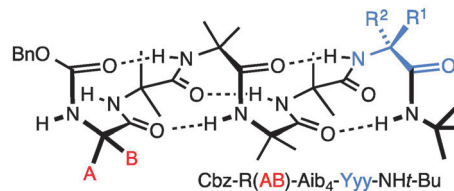
(b) Varying the C terminus of \text{Cbz-R(AB)-Aib}_4\text{-Yyy-NHt-Bu} .
