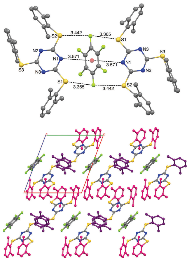
Fig. 4 X-ray structure of 2,4,6-tris(2,6-dimethylphenylthio)-1,3,5-triazine ( 6 ) crystallized in hexafluorobenzene ( 6 \cdot 0.5\text{C}_6\text{F}_6 ). The hydrogen atoms are not shown for clarity. The packing diagram of 6 \cdot 0.5\text{C}_6\text{F}_6 shows the presence of extensive inter and intramolecular \pi \cdots \pi stacking. Pink coloured dimethylphenyl rings are involved in both inter and intramolecular stacking and the purple coloured rings are involved in the intermolecular stacking. \pi \cdots \pi interactions: 4.100 Å (intra, pink); 4.160 Å (inter, pink); 4.280 Å (inter, purple).
