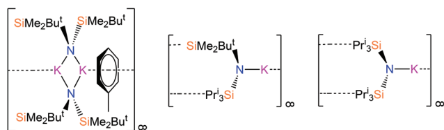
Fig. 1 The potassium silylamide complexes [\{\text{K}\{\mu\text{-N}(\text{SiMe}_2\text{Bu}^t)\}_2\text{-}(\text{C}_7\text{H}_8)\}_\infty] , [\text{K}\{\text{N}(\text{SiPr}^i)_3\}\text{-}(\text{SiMe}_2\text{Bu}^t)\}_\infty] and [\text{K}\{\text{N}(\text{SiPr}^i)_2\}_\infty] . 28
