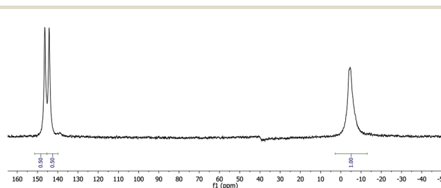
Fig. 4 ^{31}\text{P} NMR spectrum of supported phosphine–phosphite L_8 clearly showing the presence of both epimers in a 1 : 1 ratio.
