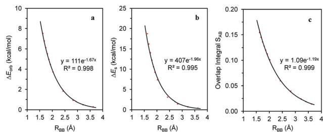
Fig. 3 Correlations of (a) \Delta E_{\text{orb}} , (b) \Delta E_s and (c) overlap integral S_{12} with the central BB bond distance in the \text{B}_4\text{H}_2 model system.
