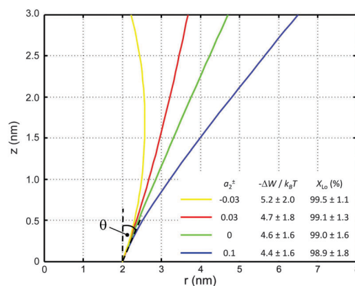
Fig. 6 Inward-bent proteins with different contours, but similar partitioning probabilities into Lo domains ( a_0 = 4\pi nm 2 , a_1^\pm = 1 nm). The inset shows the results for different a_2^\pm values.
