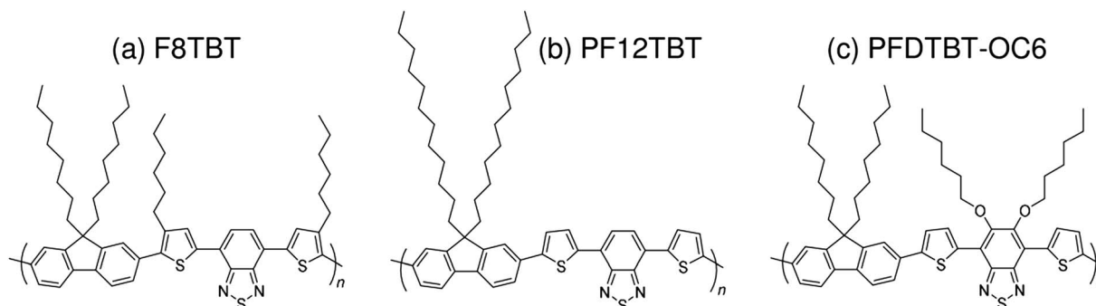
Fig. 5 Chemical structures of fluorene and BT-based polymer acceptors: (a) F8TBT; (b) PF12TBT; and (c) PFDTBT-OC6.
