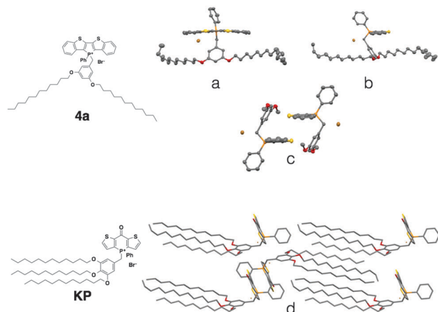
Fig. 11 Single crystal XRD data of phosphole (4a) and phosphinine-lipid (KP). (a) and (b) solid-state structures of 4a as monomers; (c) the intermolecular packing of 4a (dodecyl chains are truncated for clarity); (d) solid-state packing of KP. 9
